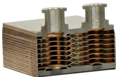
Cross-section of a brazed plate heat exchanger
